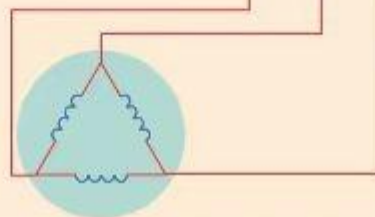
Three-phase three-wire connection
