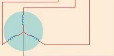
Three-phase four-wire connection
